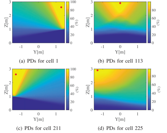
Fig. 2. Probability distributions (PDs) of coverage region and RIS location on W1 for different room cells
